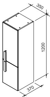
SB 350 Chrome L/R
