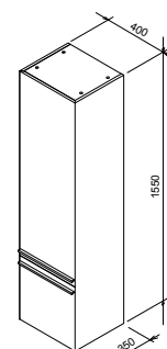
SB Clear 400 L/R
