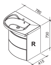
SDU Rosa Comfort 780 L/R
