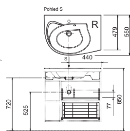
SDU Rosa Comfort 780 L/R
