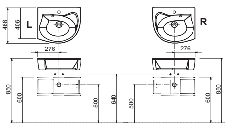
SDU Rosa 560 L/R
